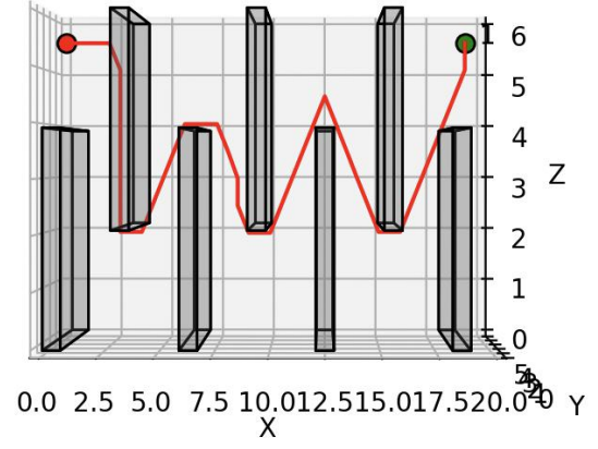
(b) ARA* on env 3
